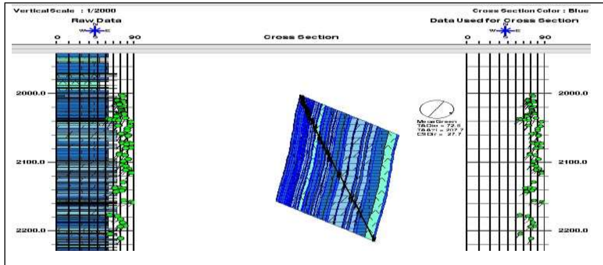
Fig. 10 Bedding dips indicating an average dip of 75 degrees S28W and strike N62W-S62E. Schematic computer generated model using dip data.
