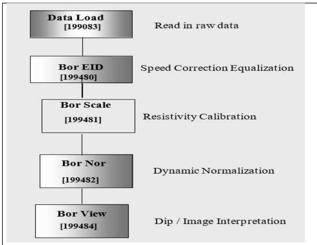
Fig. 5: Flowchart of structural and fracture analysis from FMS.
