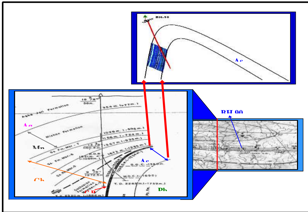
Fig. 11. Bedding dips indicating an average dip of 75 degrees S28W and strike N62W-S62E. A computer based cross-section along a NNE-SSW plane in Strucview based on this dip data matching well with NISOC structural model.
