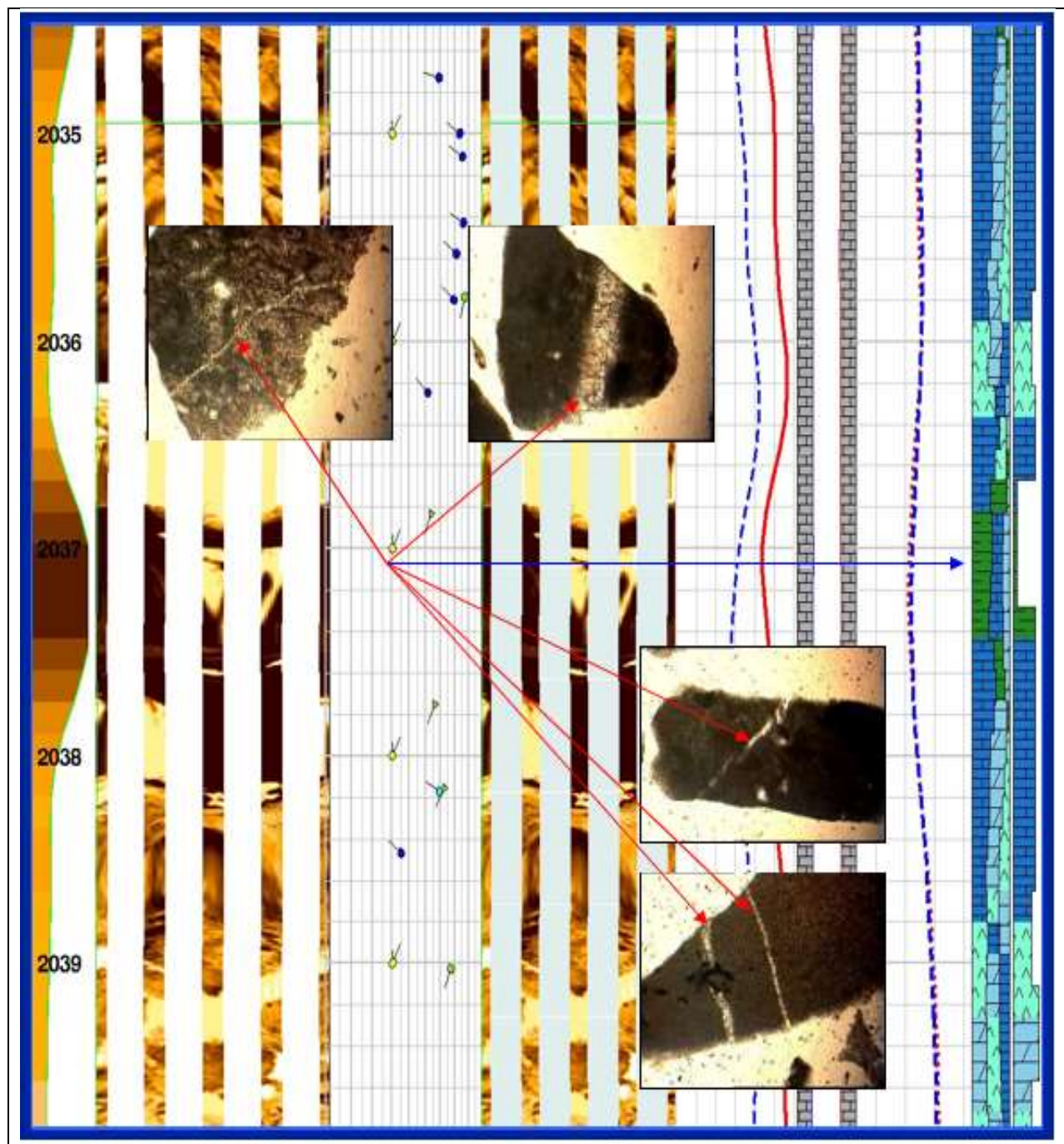
Fig. 21: Medium open fractures cemented with calcite showing in thin section of 2037m depth ,but it can not see in FMS image.
