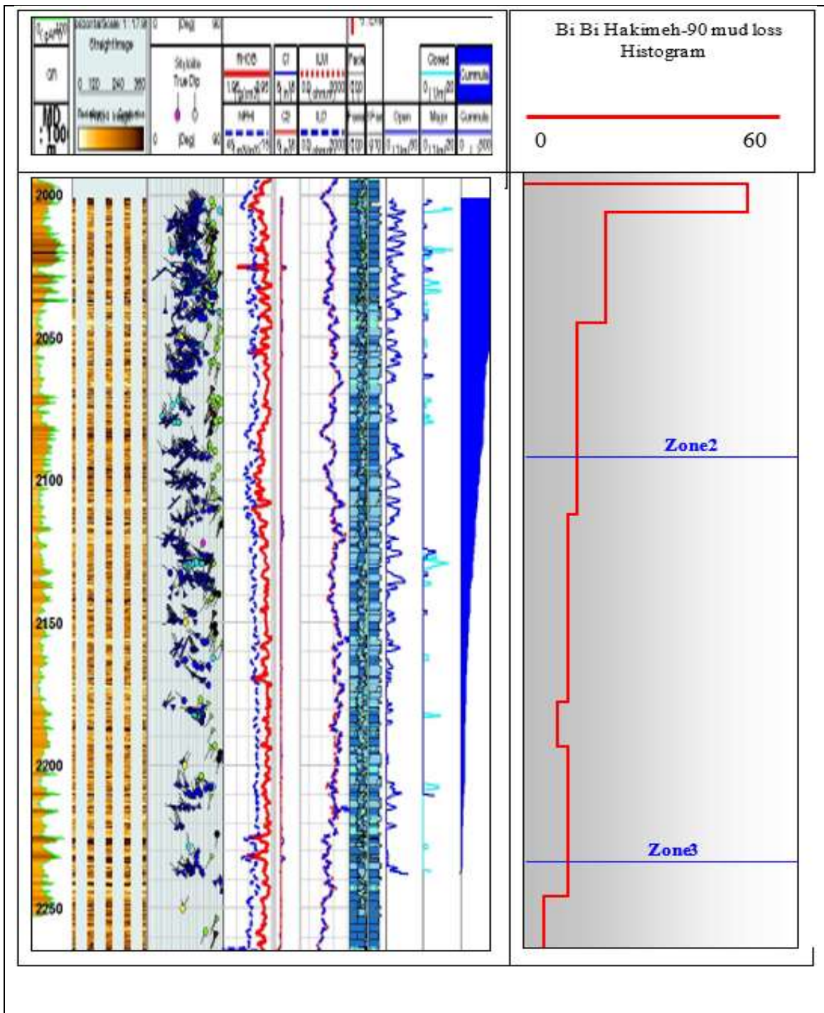
Fig. 24: Calibration of FMS fracture density data with mud loss data in Asmari reservoir. The red color is cumulative mud loss data and the blue color is cumulative fracture density data.
