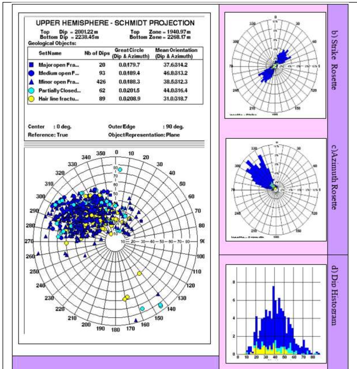
Fig. 14: Statistical plots for dips of all open fractures in the Asmari formation.
