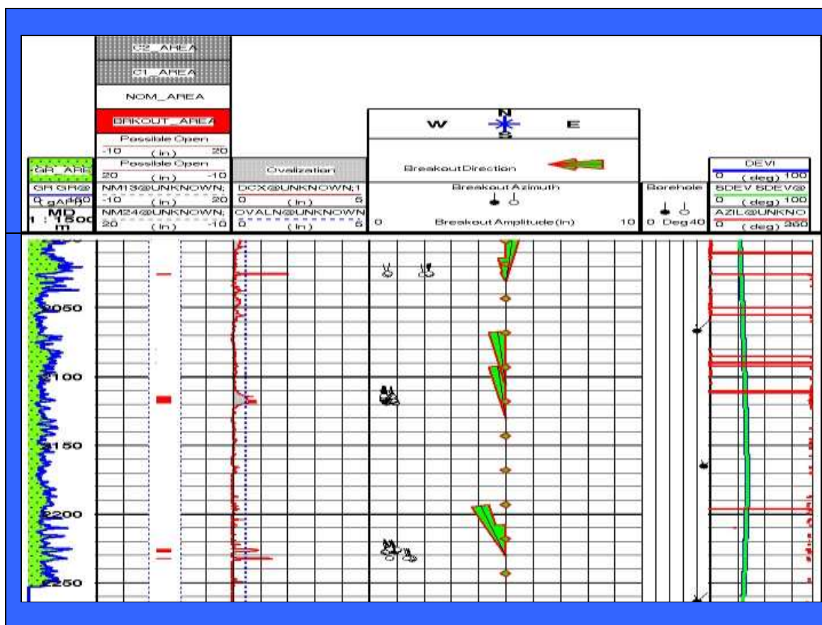
Fig. 25. In-situ stress orientations determined based on borehole breakouts identified in well BH-90. FMS images and caliper data show borehole breakouts oriented on the average NW-SE which is parallel to the minimum horizontal stress orientation.
