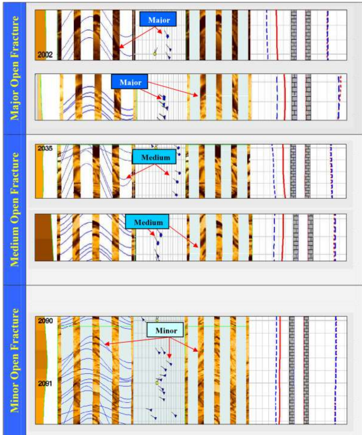
Fig. 13: Minor open fractures (blue triangle dips), Medium open fractures (blue circular dips) and Major open fractures (blue square dips) are shown by FMS image in Asmari formation.
