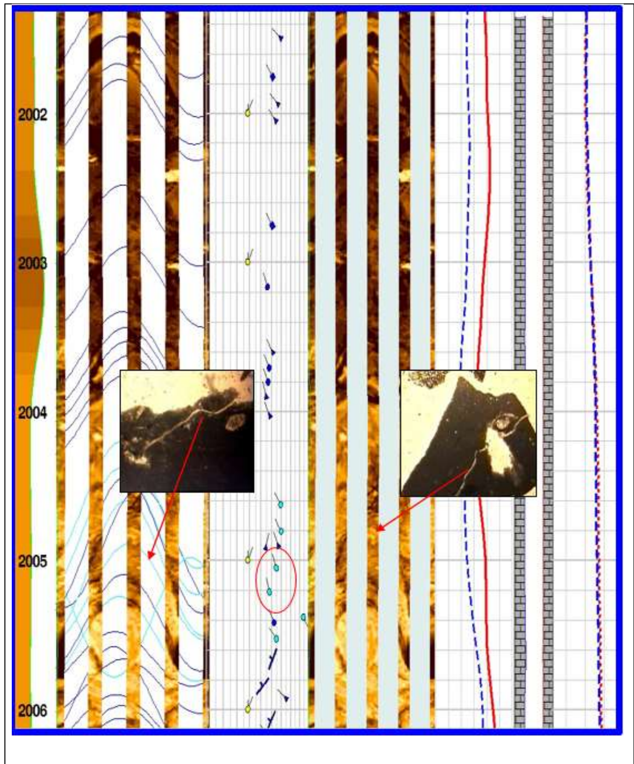
Fig. 19: Minor open fractures (partially cemented) with calcite showing in thin section of 2005m depth.
