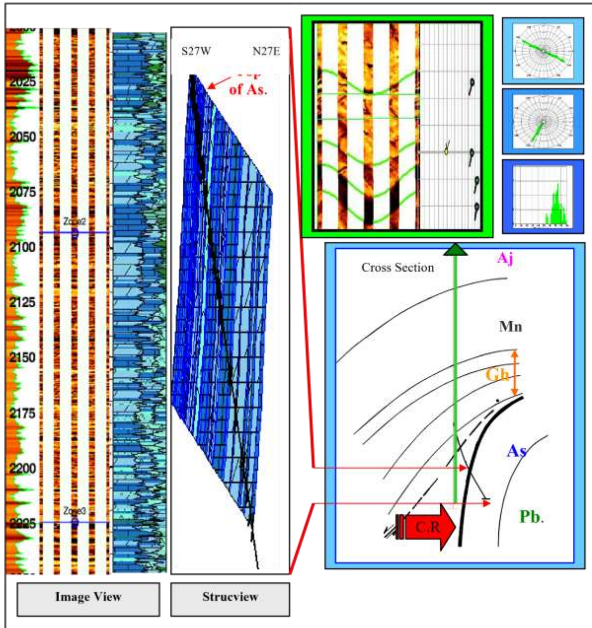
Fig. 12. Composite plot of orthogonal calipers (C1 and C2), GR, FMS static normalized images, dips, well deviation, bedding dip, and lithology in Asmari formation. . Bedding dips indicating an average dip of 75 degrees S28W and strike N62W-S62E. A computer based cross-section along a NNE-SSW plane in Strucview based on this dip data matching well with NISOC structural model.
