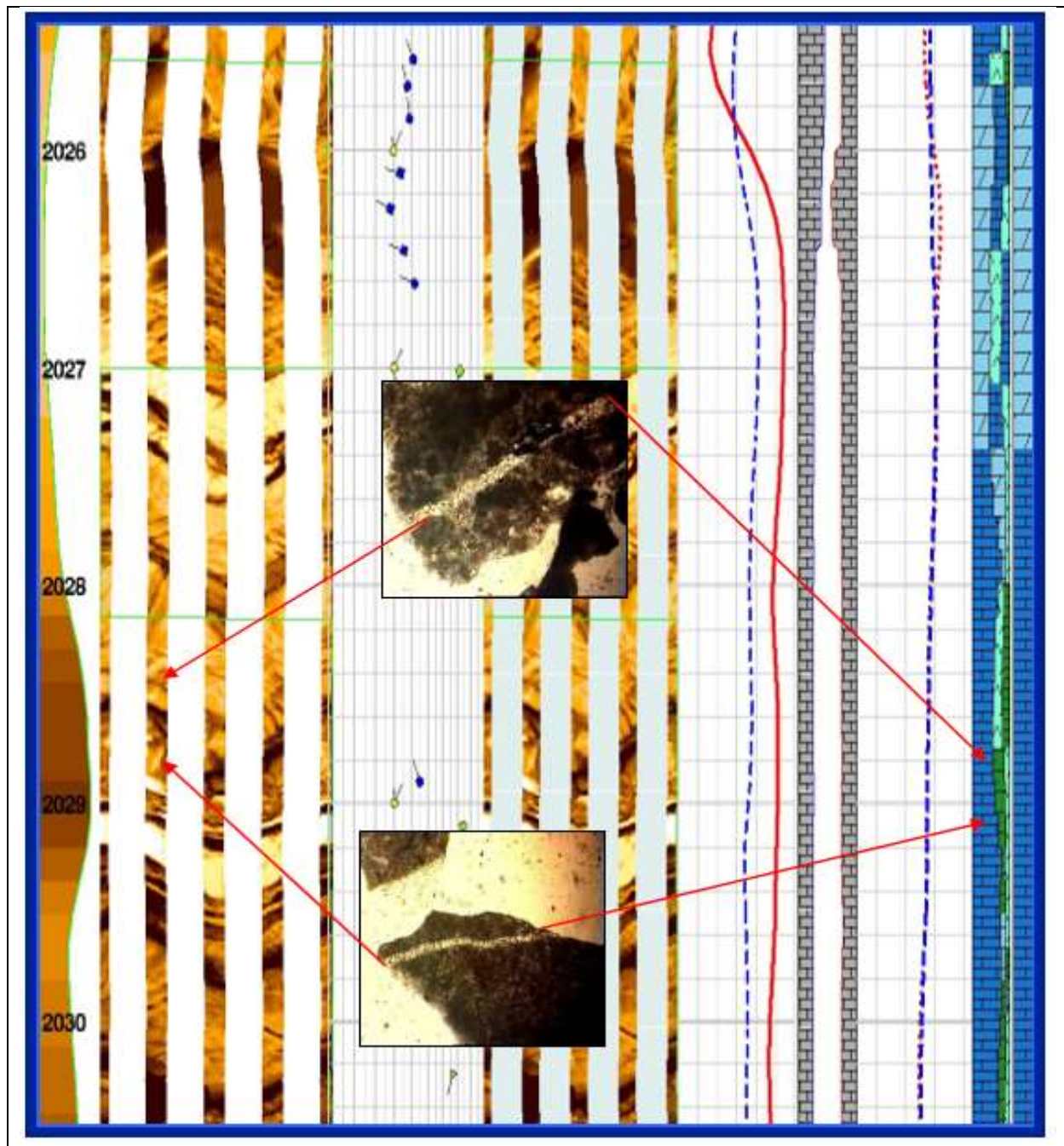
Fig. 20: Medium open fractures cemented with calcite showing in thin section of 2029m depth and it has good match with FMS Image in shaly limestone layers.
