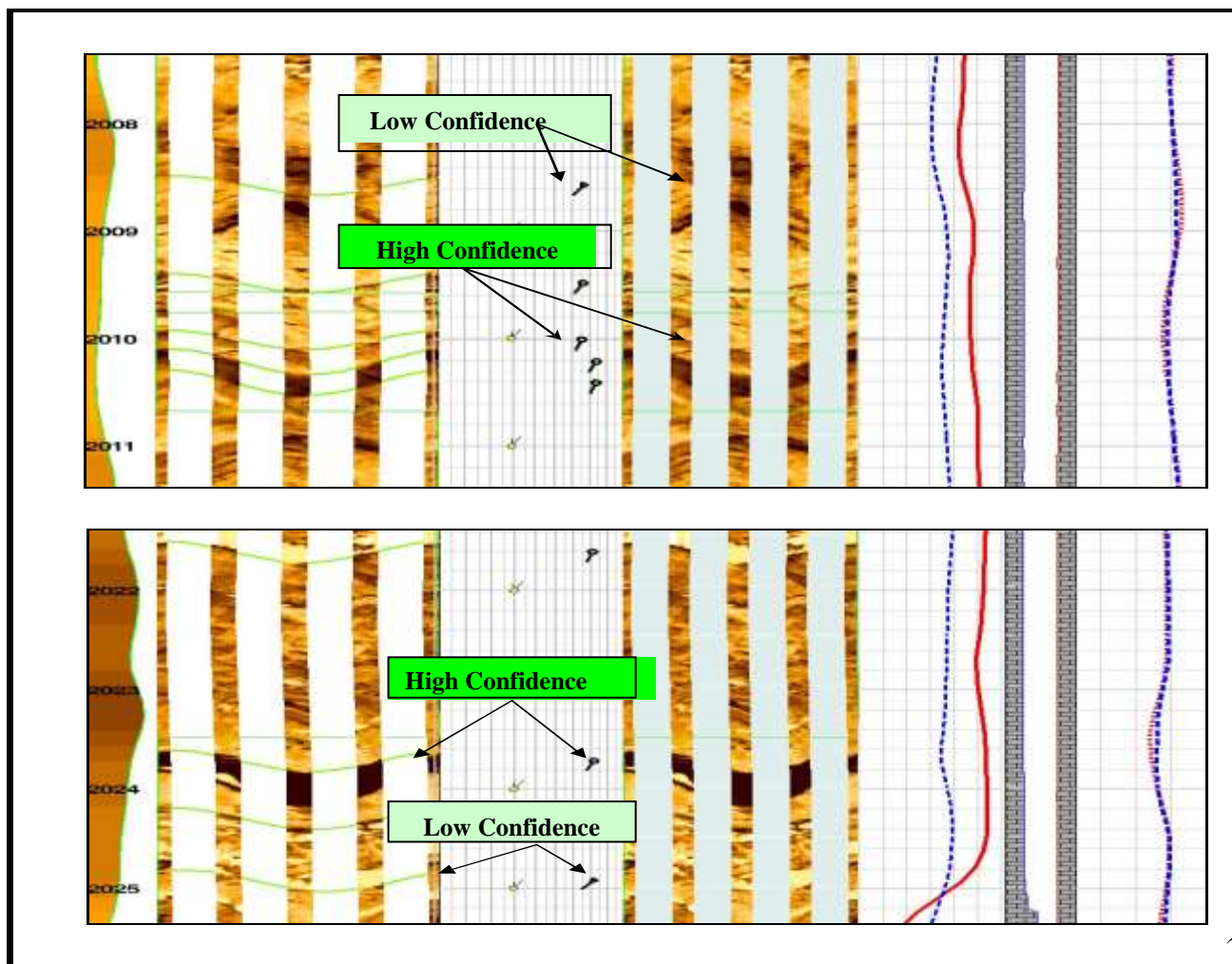
Fig. 6: The dips corresponding to layer / bed boundaries are shown as low and high confidence based on their sharpness and planarity for computation of structural dip.
